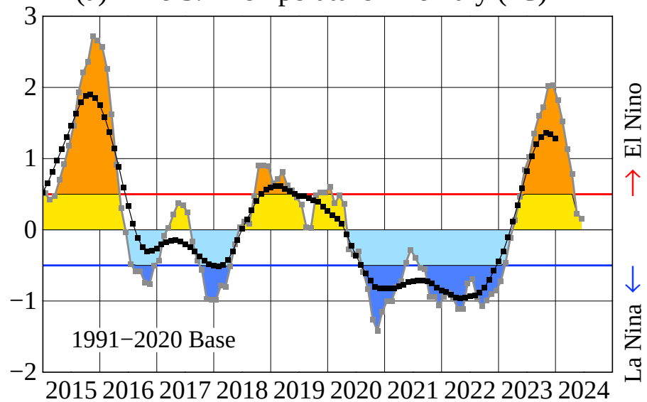
(a) Nino 3.4 Temperature Anomaly ( ^{\circ}\text{C} )
