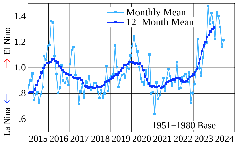
(b) Global Temperature Anomaly ( ^{\circ}\text{C} )
