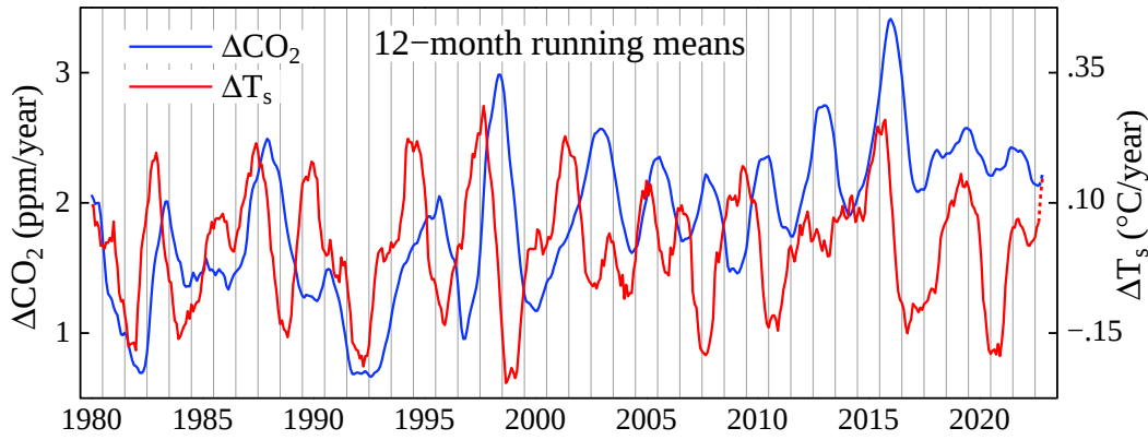
Annual Growth of Global CO 2 and Surface Temperature
