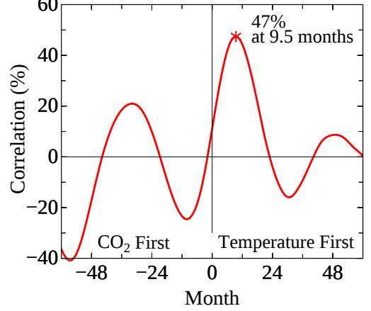
Correlations of CO 2 with Temperature
