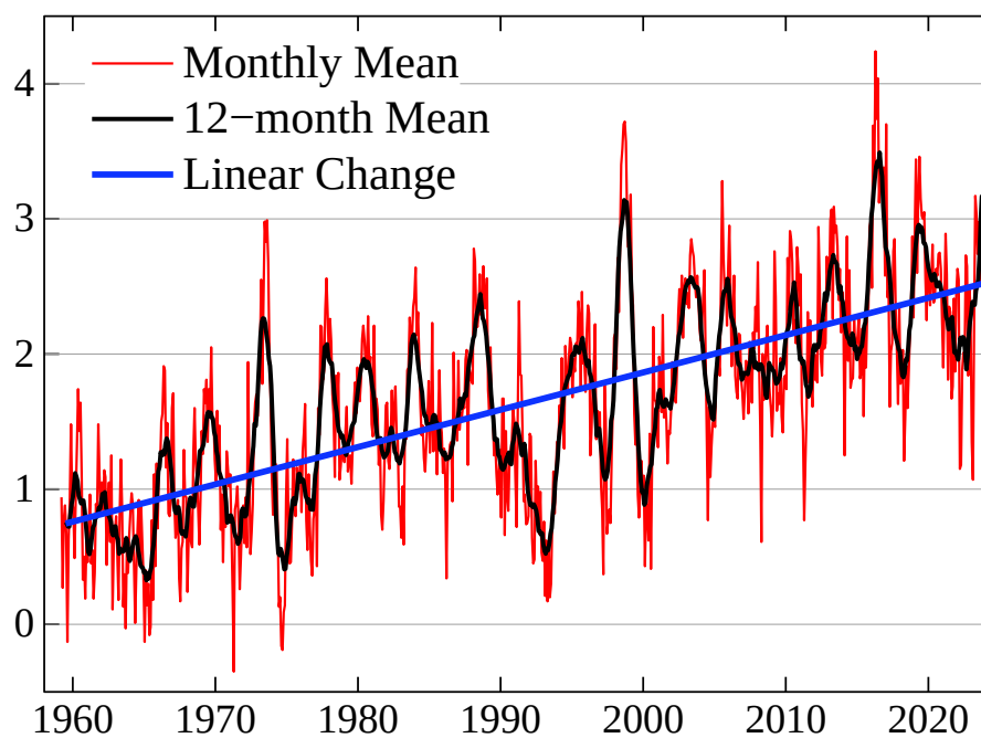
CO 2 Increase (ppm/year) at Mauna Loa
