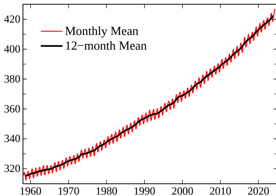
Atmospheric CO 2 (ppm) at Mauna Loa
