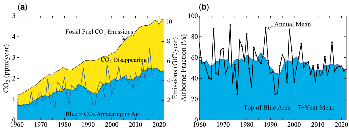
Figure 26. Fossil fuel emissions divided into portions appearing in the annual increase of airborne CO 2 and the remainder, which is taken up by the ocean and land (1 ppm CO 2 ~ 2.12 GtC).
