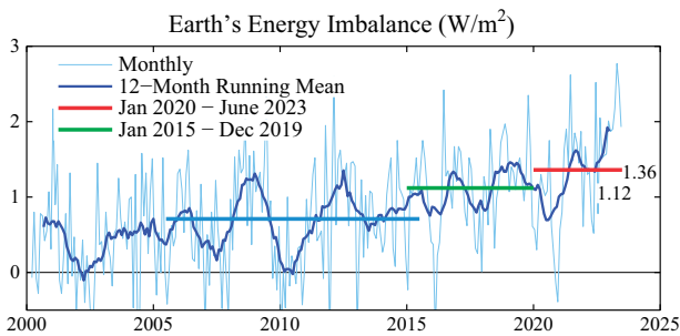
Figure 25. 12-month running-mean of Earth's energy imbalance from CERES satellite data [81] normalized to 0.71 W/m 2 mean for July 2005–June 2015 (blue bar) from in situ data [80].
